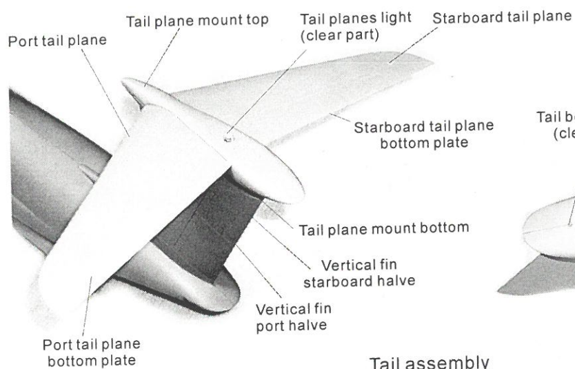
Tail assembly
