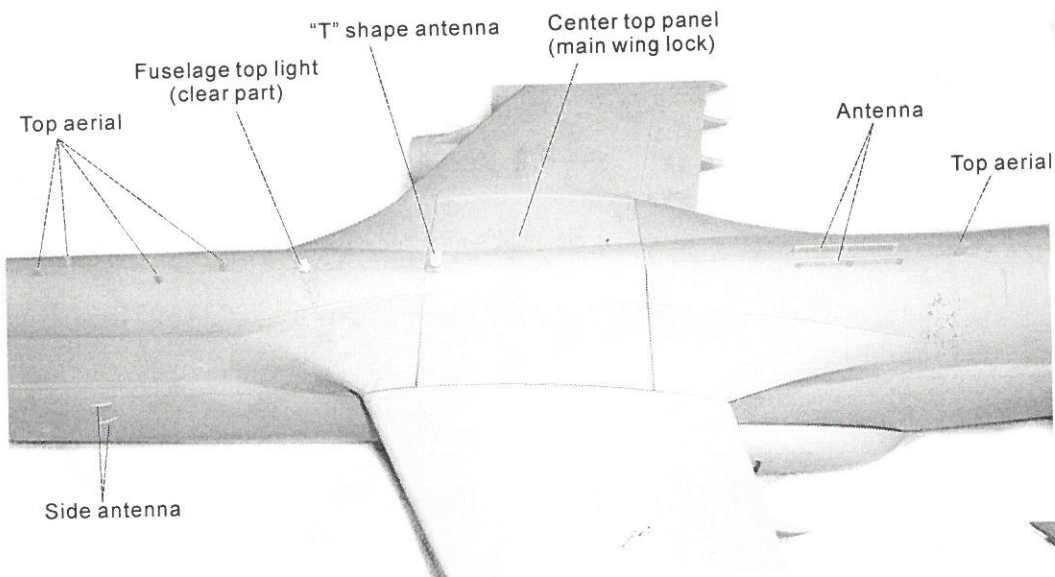
Fuselage top assembly
